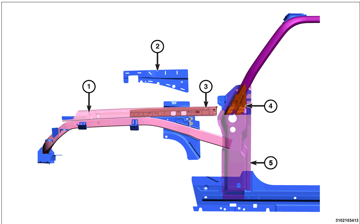
Upper Load Path Beam And A-pillar Composite Reinforcements
