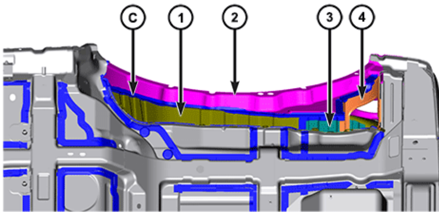
Inner Wheelhouse- Left (3 of 3)
