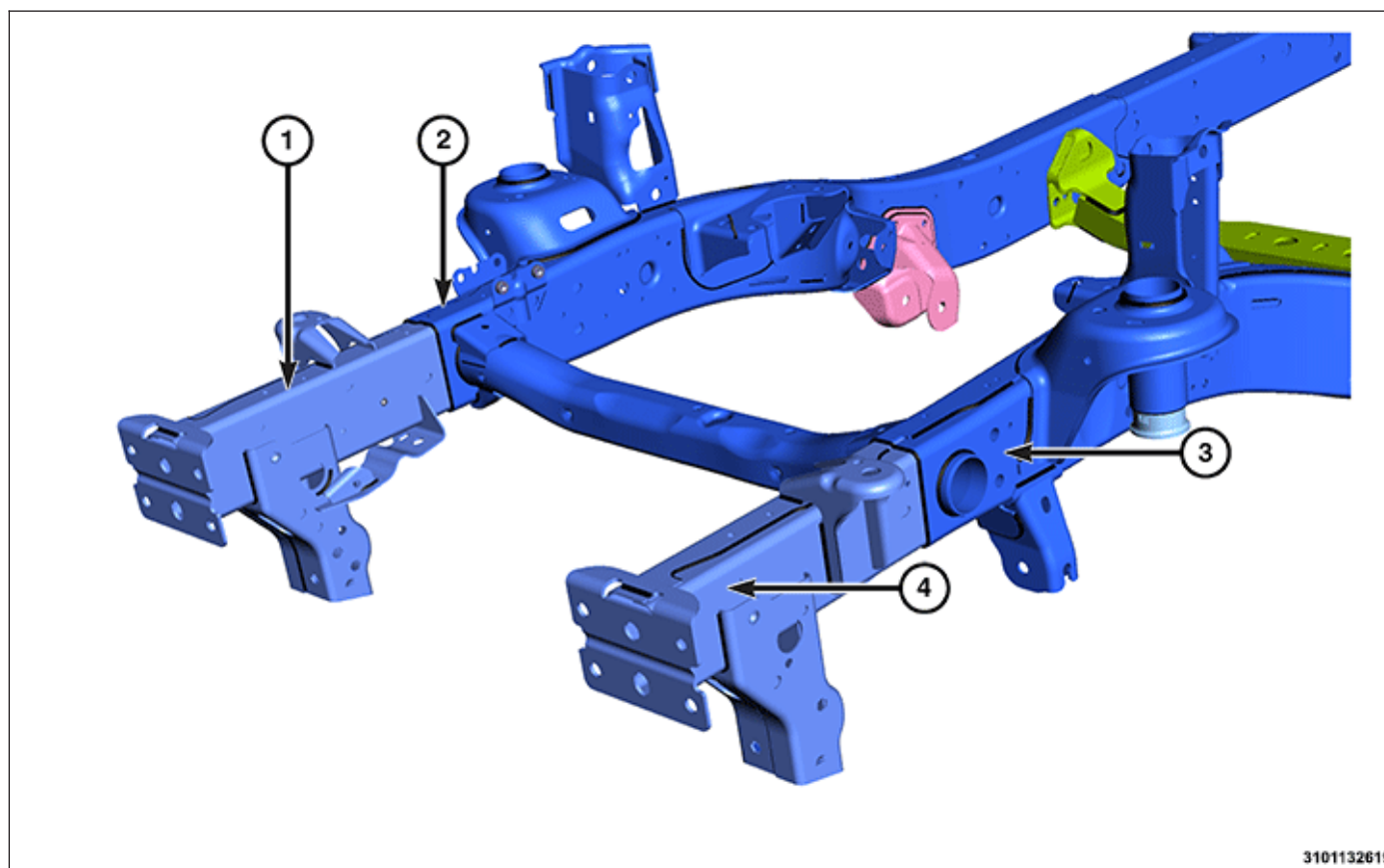
Front Frame Rail Extensions
