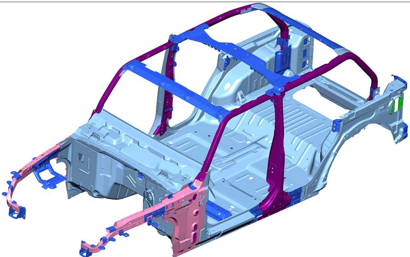
Body In White (Top view front) - JL 74 (4 Door)
