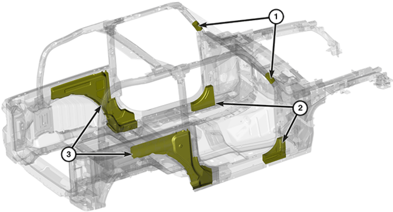
PUR Foam Locations JL 72 (2 Door)
