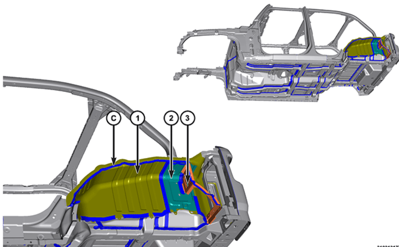
Inner Wheelhouse- Left (2 of 3)
