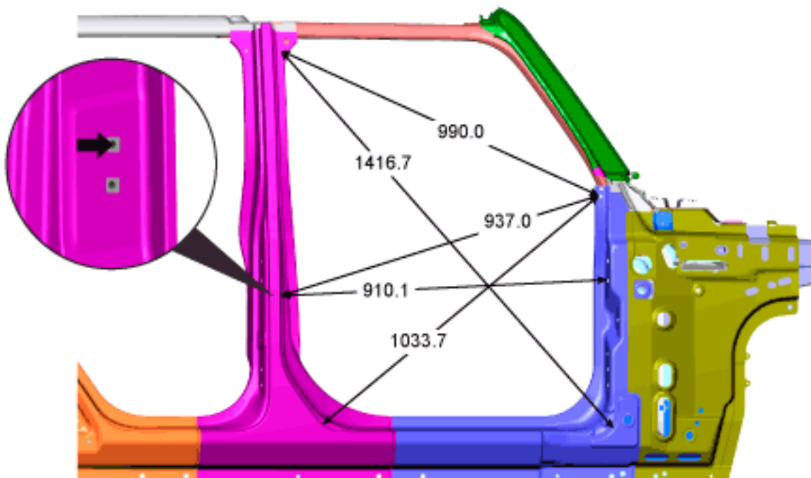
Front Door Opening- JL 72 (2 Door)
