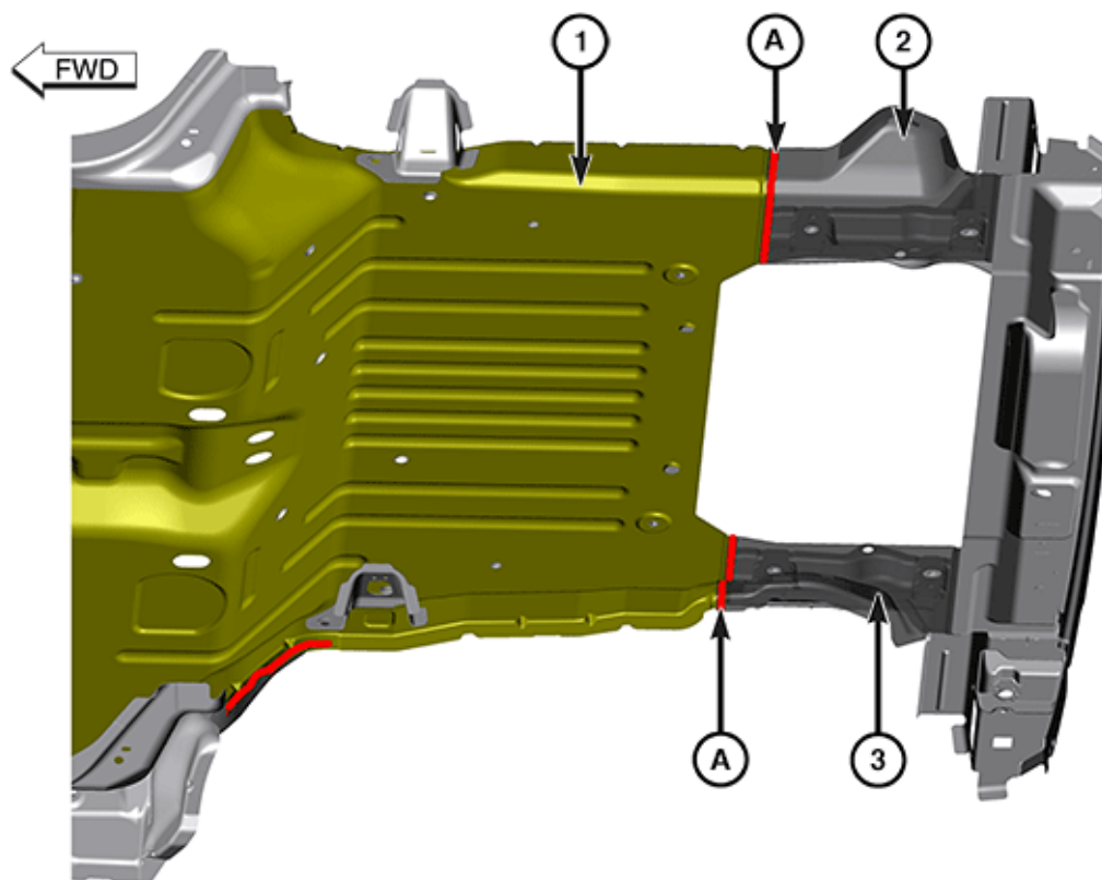
Rear Floor (Transparent for Clarity)
