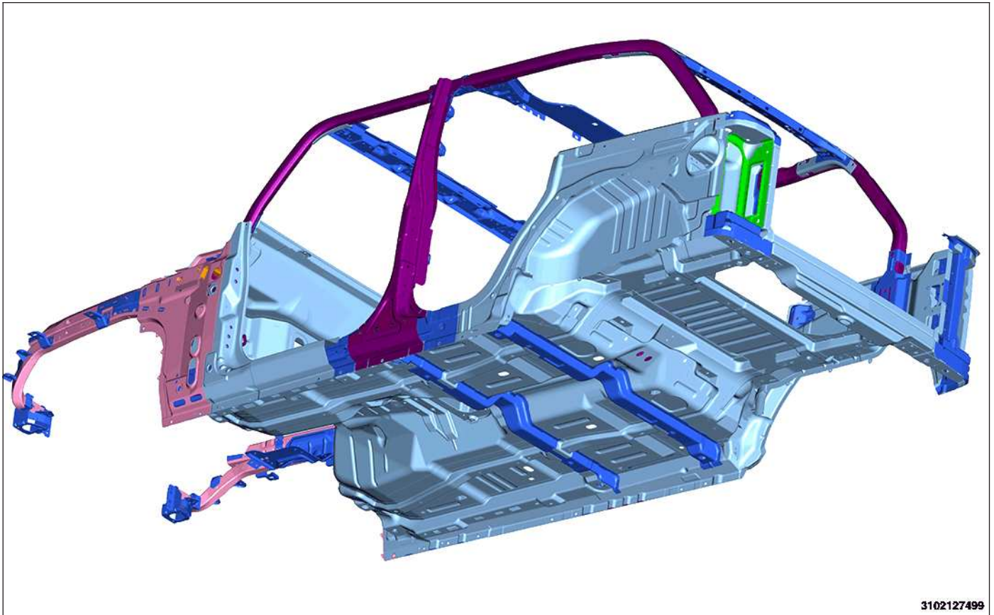
Body In White (Bottom view rear) - JL 74 (4 Door)
