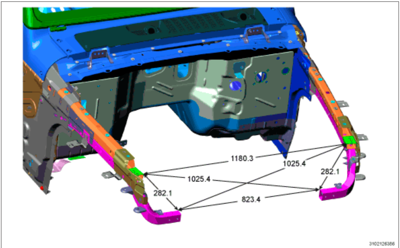
Under Hood Dimensions (2 of 2)
