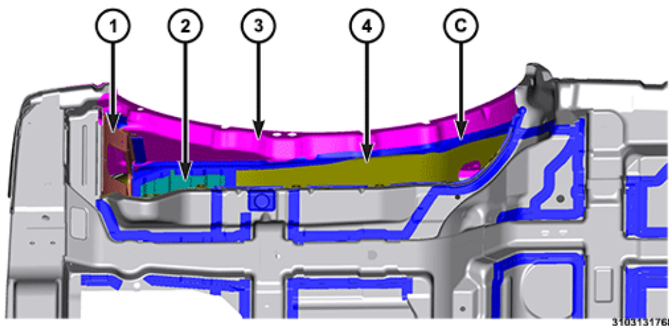
Inner Wheelhouse- Right (3 of 3)
