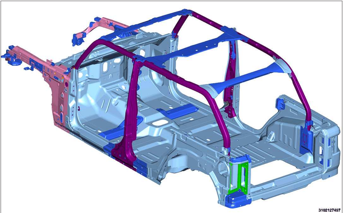
Body In White (Top view rear) - JL 74 (4 Door)
