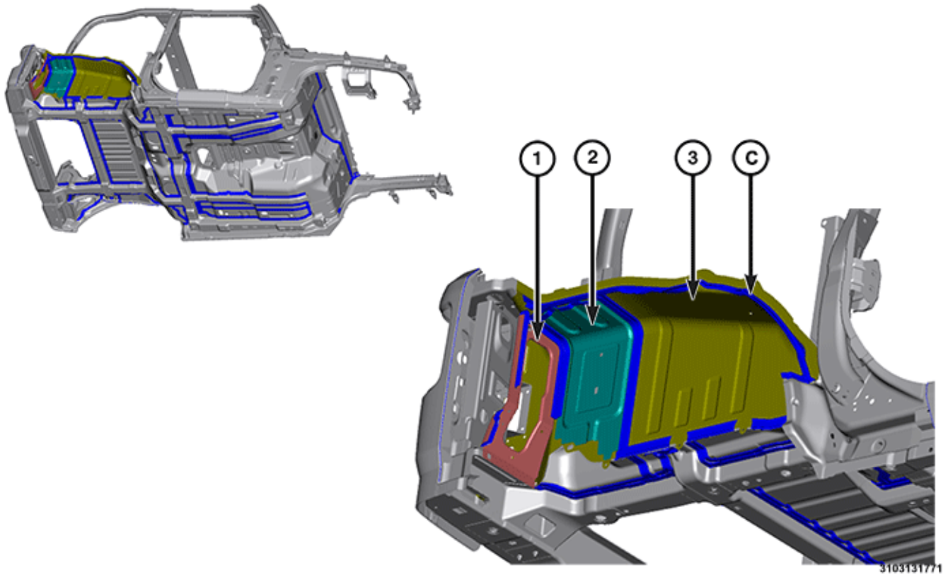
Inner Wheelhouse- Right (2 of 3)
