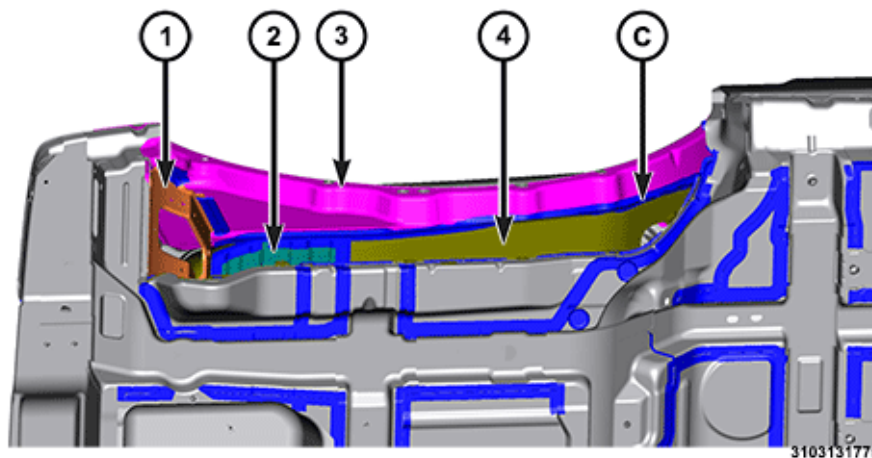
Inner Wheelhouse- Right (3 of 3)
