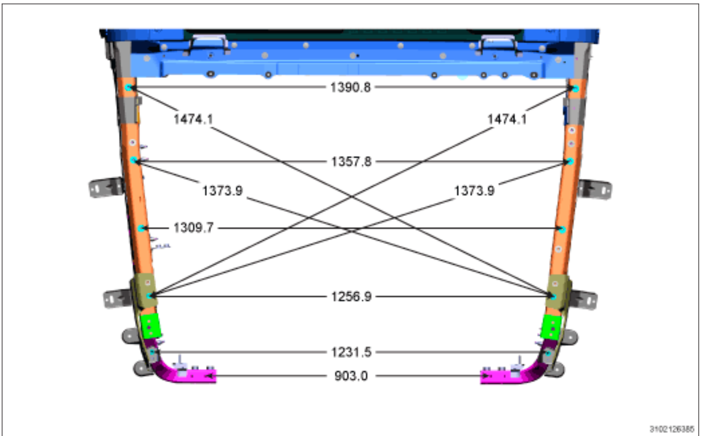
Under Hood Dimensions (1 of 2)
